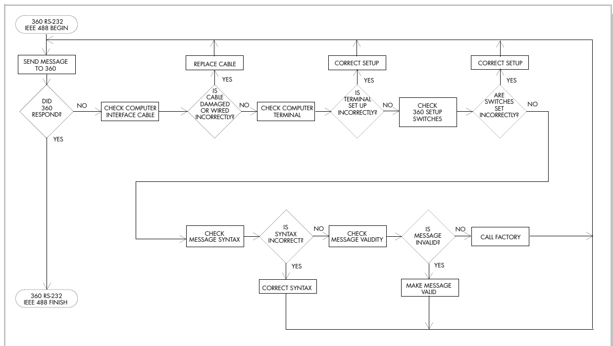
Figure 6-11 RS-232/IEEE 488 Interface.
