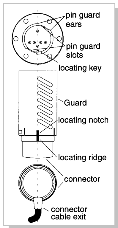
Stabil-Ion Gauge Connector Orientation (Prior to Installation).
