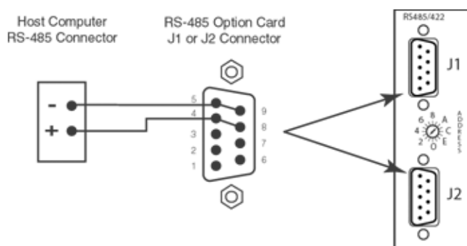
RS-485 Connectors
