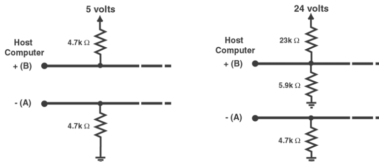
RS-485 Bias Resistor
