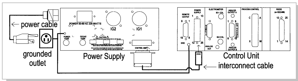
Power Supply and Control Unit Rear Views Showing Power Cable Connections.
