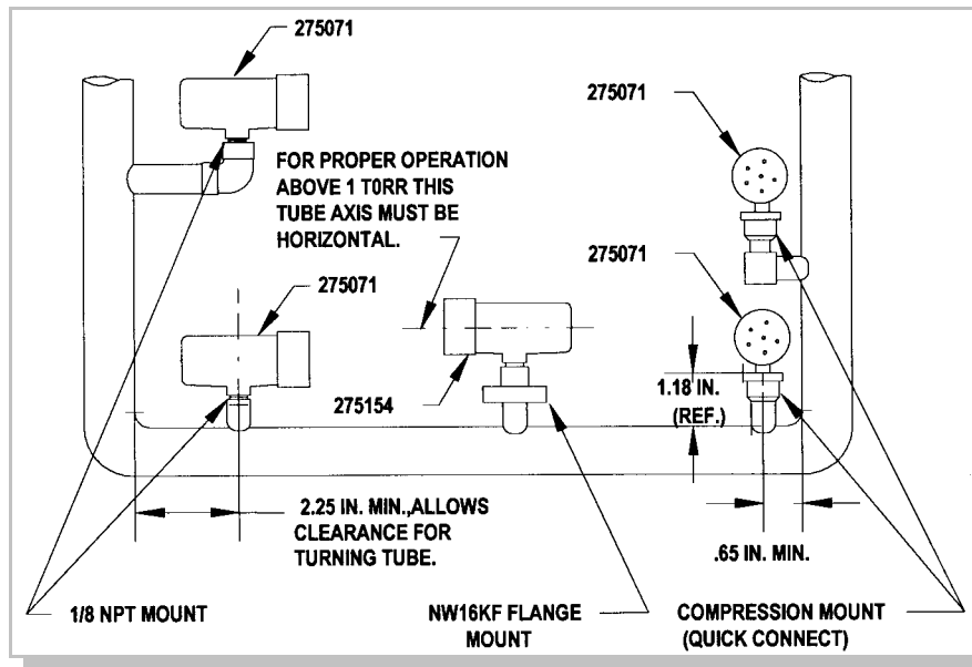
Figure 3-4 Convectron Gauge Installation.
