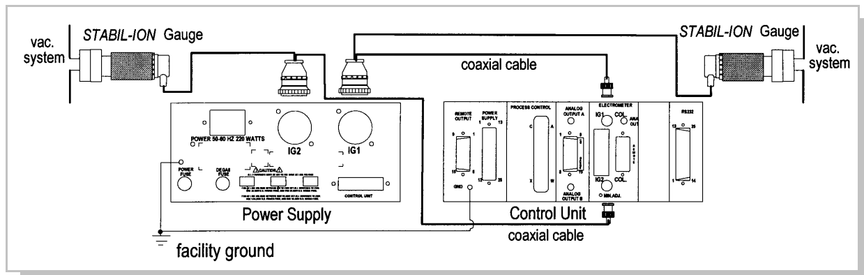
Power Supply and Control Unit Rear Views Showing the Cable Connections to the Stabil-Ion Gauges.
