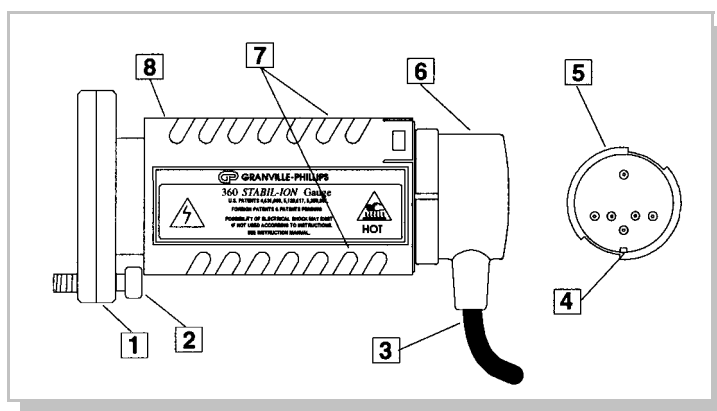
Figure 1-2 Stabil-Ion Gauge.
