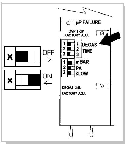
Figure 2-22 Top View of Electrometer Module Showing Degas Time Switches.
