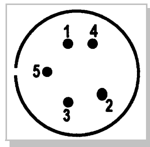
Figure 6-5 Convector Gauge Base.
