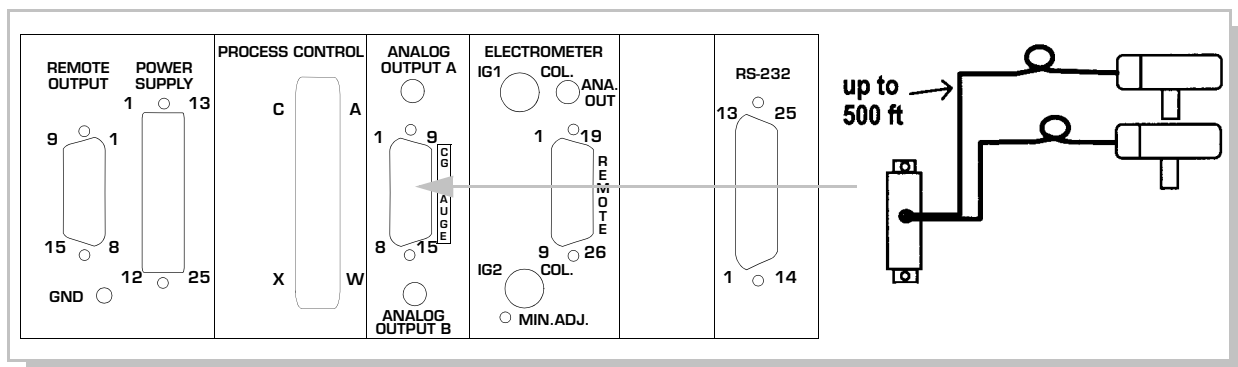
Control Unit Rear Panel Showing the Cable Connection to the Convector Gauges.
