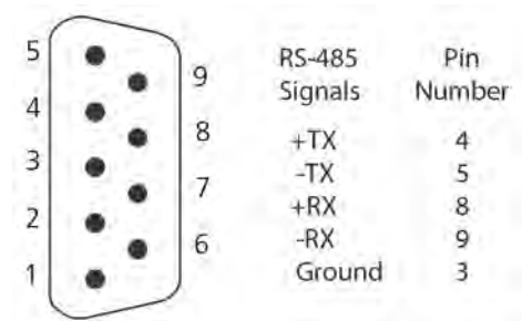
RS-485 Connector
